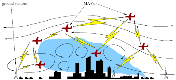
Figure 1. An airborne WSN for 3-D sensing of toxic plumes.
