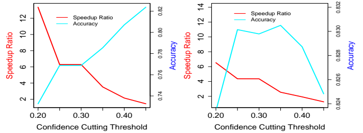
Figure 7: Optimal cascaded classifier performance by the (L) BAST criterion and by the (R) BFA criterion.
