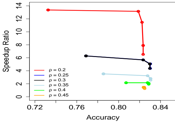
Figure 8: Optimal cascaded classifier performance on different control balance and confidence threshold.
