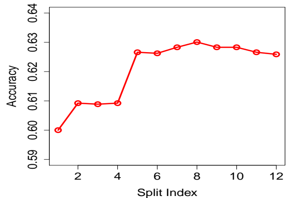
Figure 3: Classification accuracy of the CR algorithm on mobile video chat data using different split thresholds.
